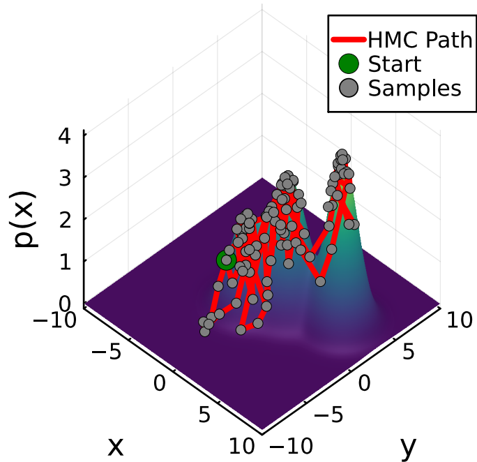
HMC Trajectory
